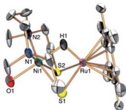
Fig. 3. Structure of [2](NO 3 ) as determined by neutron diffraction analysis. The ellipsoids are cut open to reveal the three principal axes and are drawn to include 30% probability density. Selected bond lengths (Å) and angles (°): Ni1–H1, 1.859 ± 0.007; Ni1–O1, 2.122 ± 0.005; Ni1–S1, 2.359 ± 0.010; Ni1–S2, 2.362 ± 0.009; Ni1–N1, 2.119 ± 0.003; Ni1–N2, 2.117 ± 0.004; Ru1–H1, 1.676 ± 0.008; Ru1–S1, 2.375 ± 0.011; Ru1–S2, 2.388 ± 0.007; Ni1–H1–Ru1, 101.47 ± 0.043; Ni1–S1–Ru1, 70.7 ± 0.3; and Ni1–S2–Ru1, 70.4 ± 0.2.
